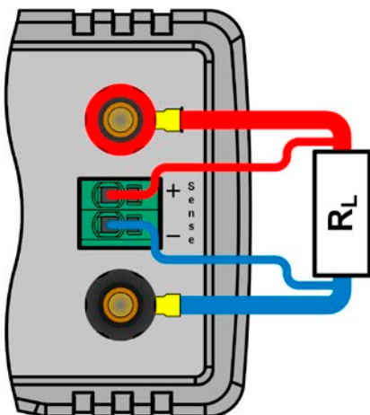
Figure 13 - Principle example for remote sensing wiring
